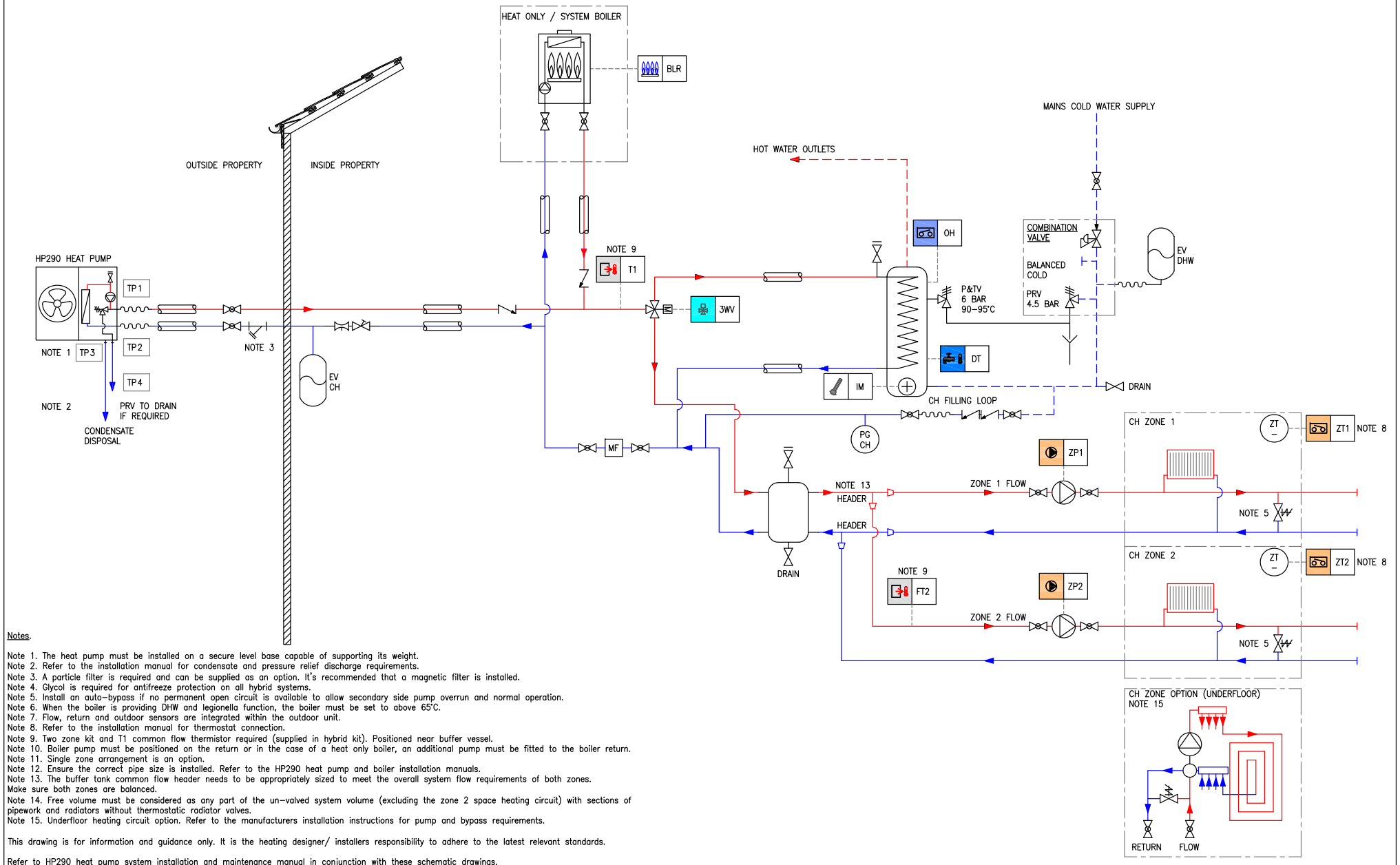
Figure 15. HP290 + System Boiler + DHW + Two Zones (Bivalent System)
