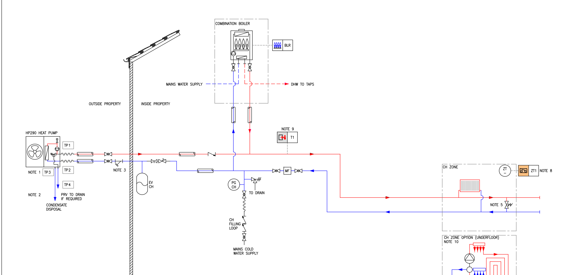
Figure 13. HP290 + Combi Boiler + Single Zone (Bivalent System)
