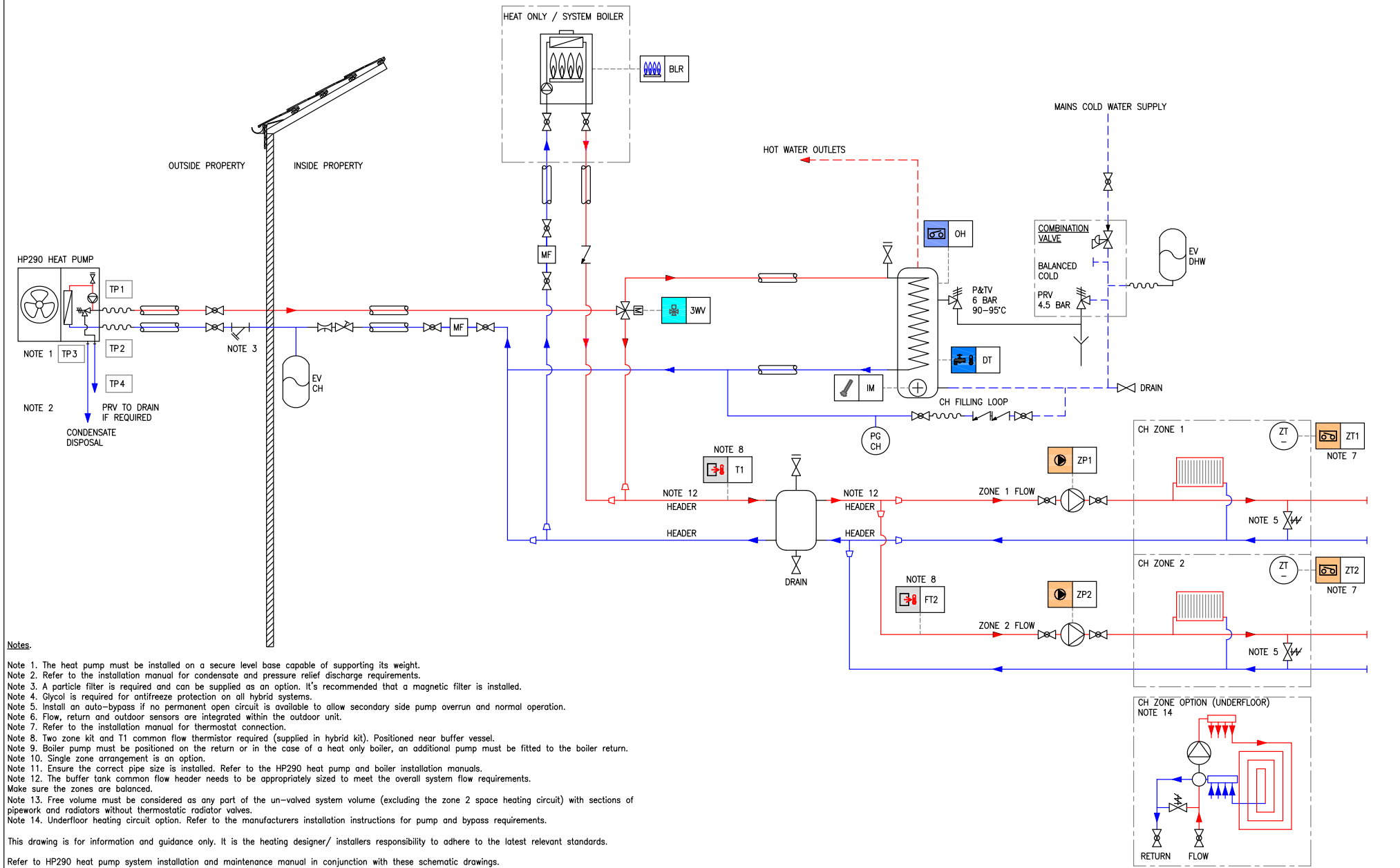
Figure 17. Hydraulically separated HP290 + System Boiler + DHW + Two Zones (Bivalent System)
