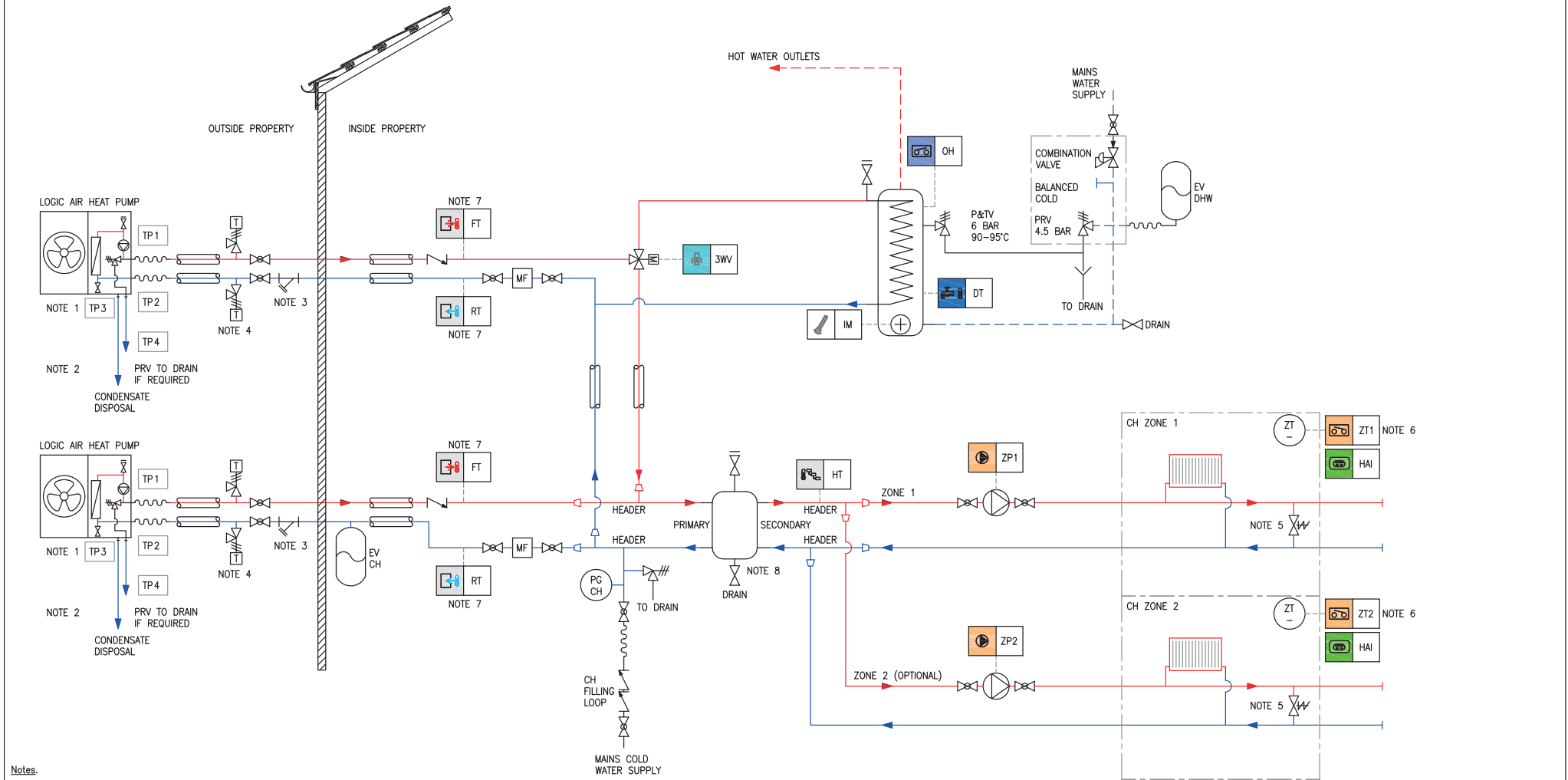
Figure 21. Logic Air Monobloc Cascade, Third Party DHW Cylinder, Decoupler with Two Zones
