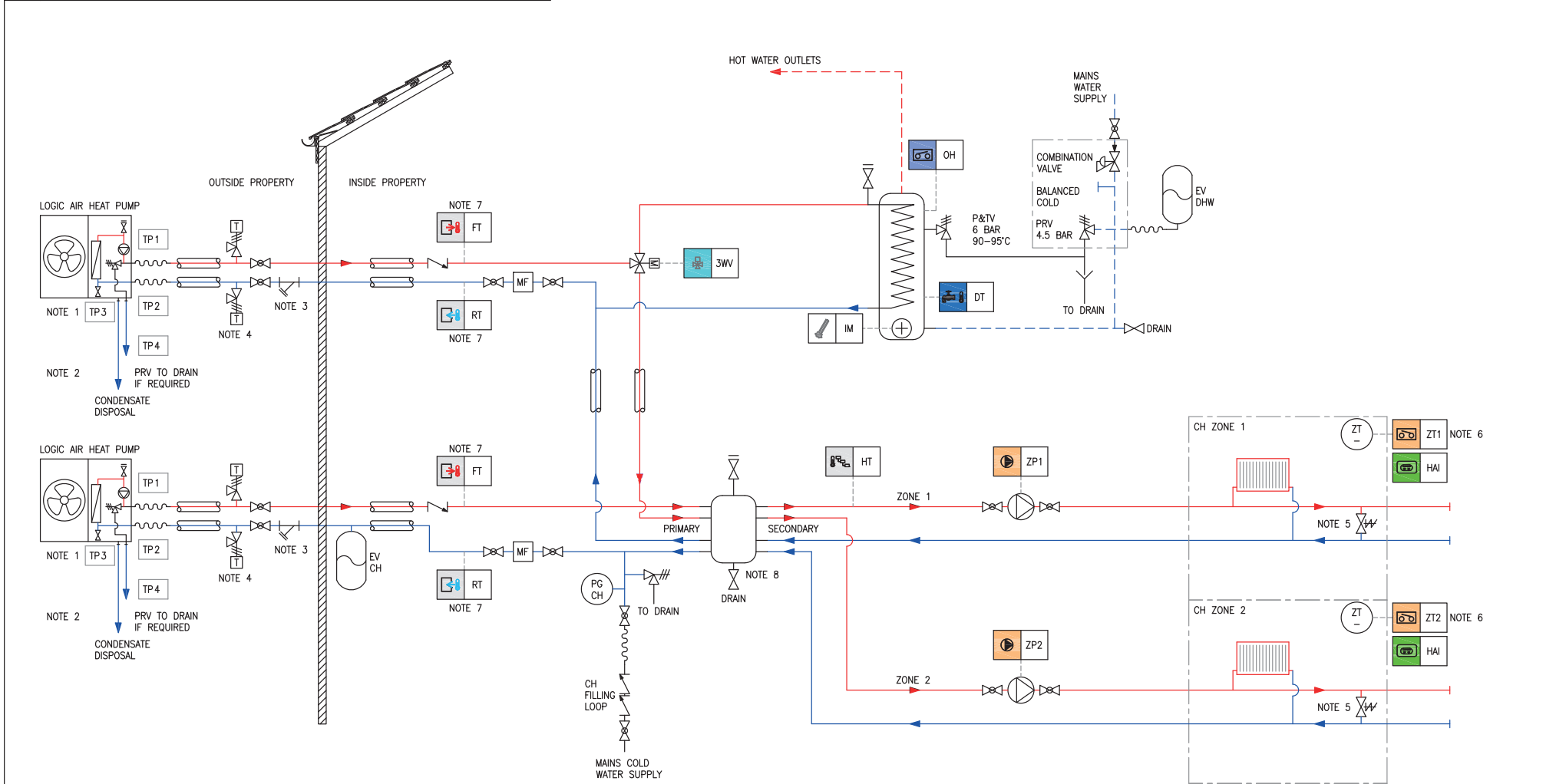
Figure 22. Logic Air Monobloc Cascade + Third Party DHW Cylinder + Multi-Port Decoupler with Two Zones
