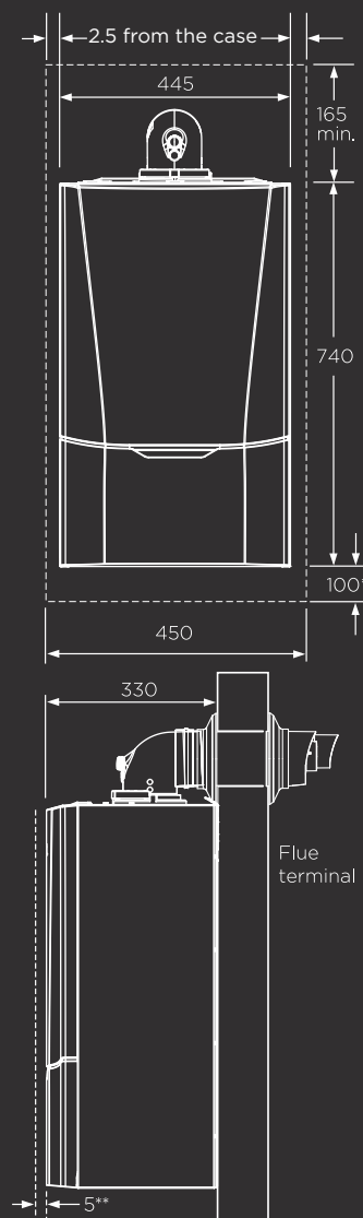
Dimensions in mm.
